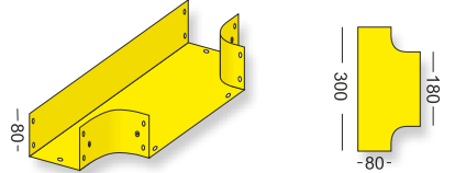
COMPONENT NAME horizontal tee 08-18 PART NO. ET-08-18
