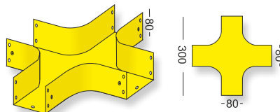
COMPONENT NAME cross 08-08 PART NO. EX-08-08
