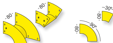
COMPONENT NAME vertical elbow- down 08-30° EŁz-08-30 vertical elbow- down 08-90° EŁz-08-90
