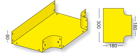
COMPONENT NAME horizontal tee 18-18 PART NO. ET-18-18
