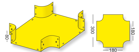
COMPONENT NAME cross 18-18 PART NO. EX-18-18
