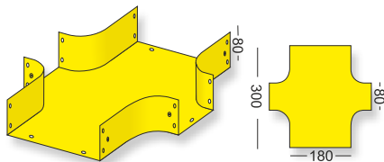
COMPONENT NAME cross 18-08 PART NO. EX-18-08
